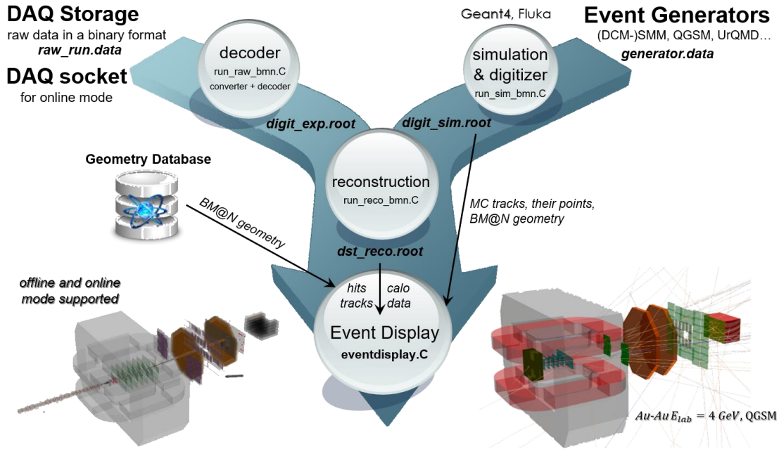
Figure 10. Input data for BM@N event display
