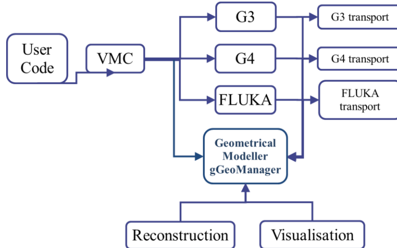
Figure 3. Geometrical Modeller (gGeoManager) for the MC simulation
