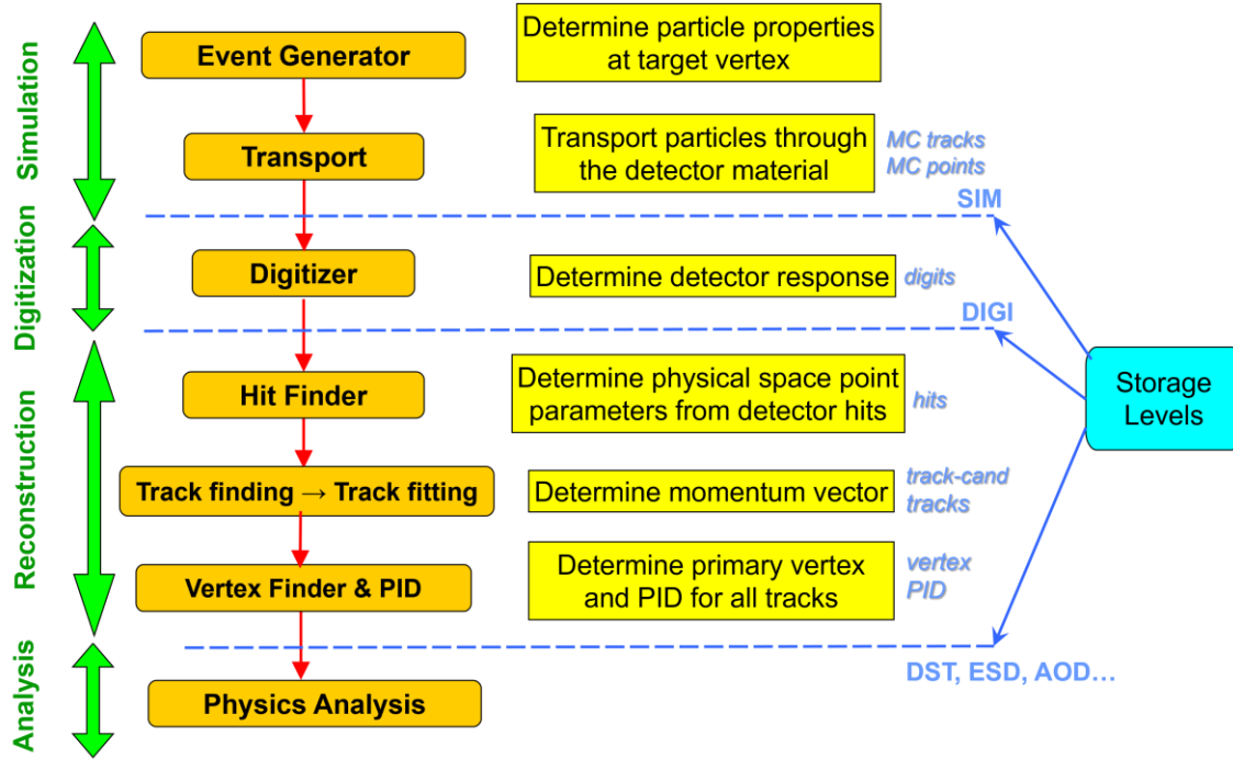
Figure 5. Data processing steps and storage levels of the BM@N experiment
