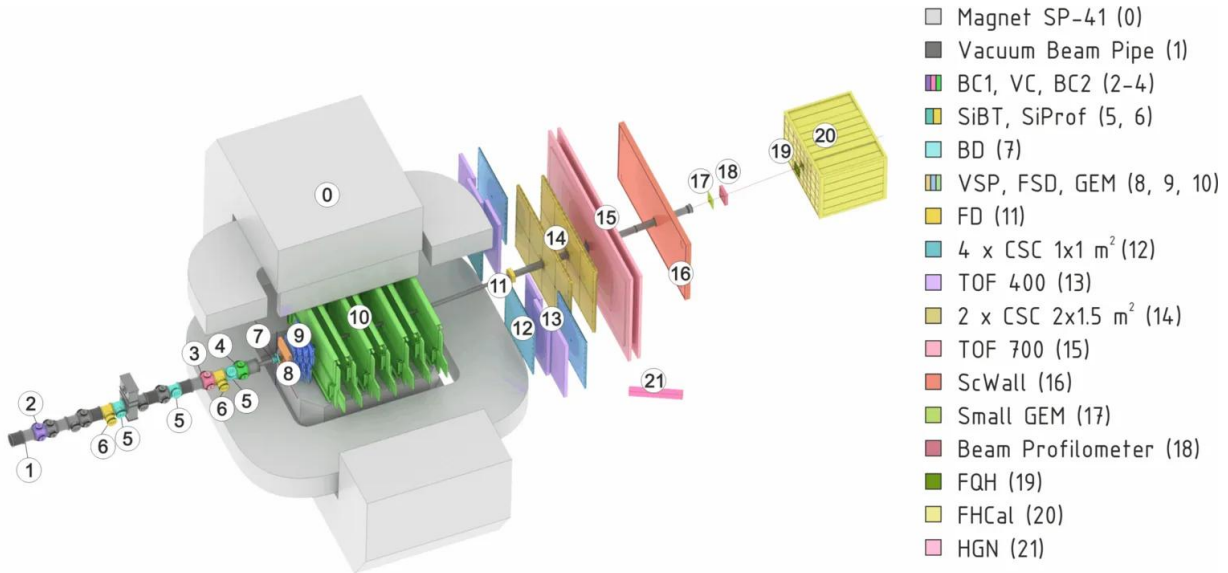
Figure 2. Scheme of the BM@N setup in Run 9
