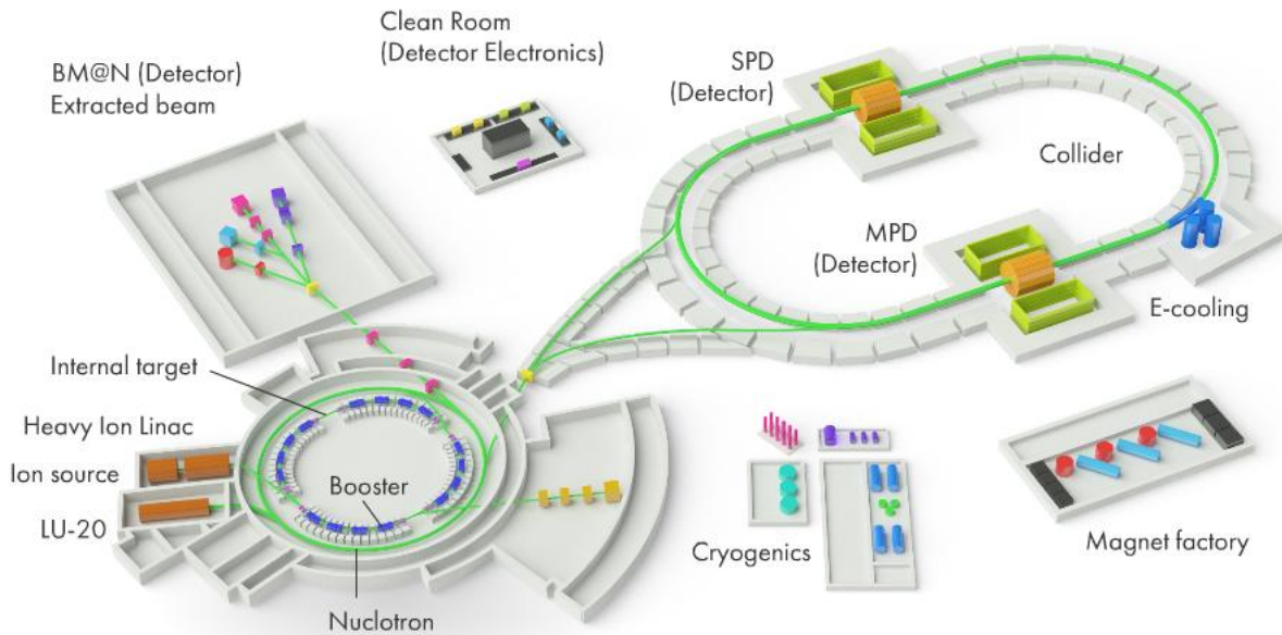
Figure 1. NICA complex with the BM@N experiment at the extracted Nuclotron beam
