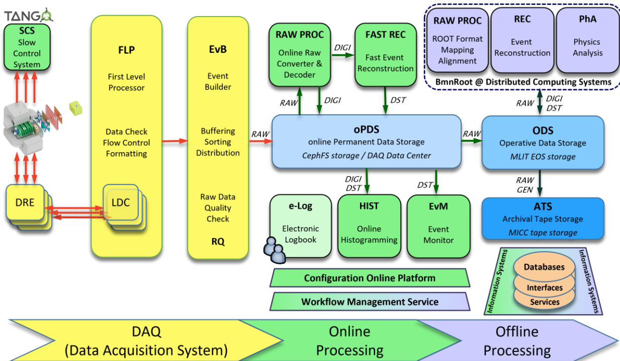
Figure 17. Data processing pipeline
