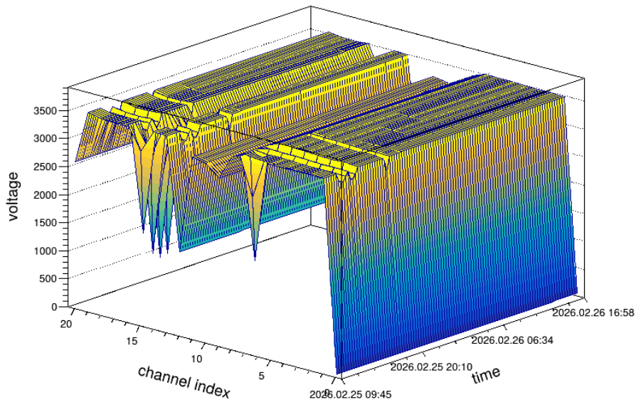
Figure 16. High voltage of the GEM channels for the runs 9696–9730 of Run 9
