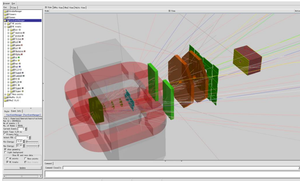
Figure 12. BM@N event visualization of MC tracks in Bi – Bi collision at 4 GeV/nucleon
