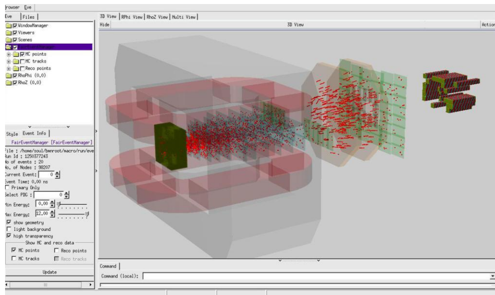
Figure 13. Event display for Bi – Bi collisions in the high transparency mode
